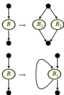
Figure 5: Examples of structured data flow equations for activity analysis
