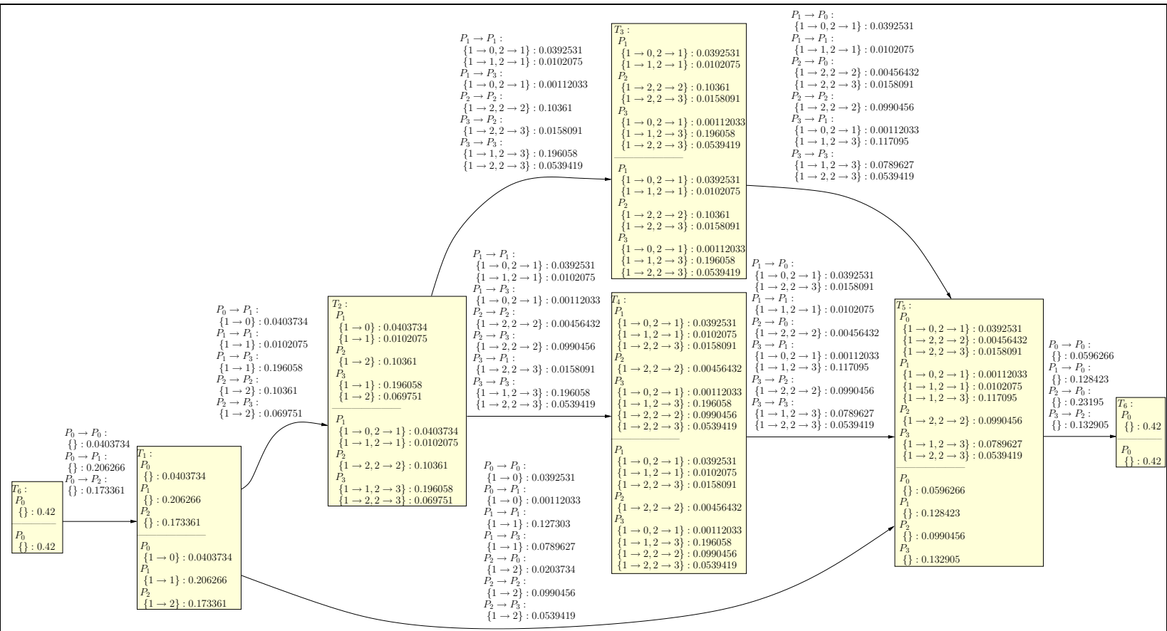
Figure 12: Solution given by the linear program : the application graph is annotated with the non-zero values of cons(P_i, T_k^L) , prod(P_i, T_k^L) , sent(P_i \rightarrow P_j, e_{k,l}^L)
