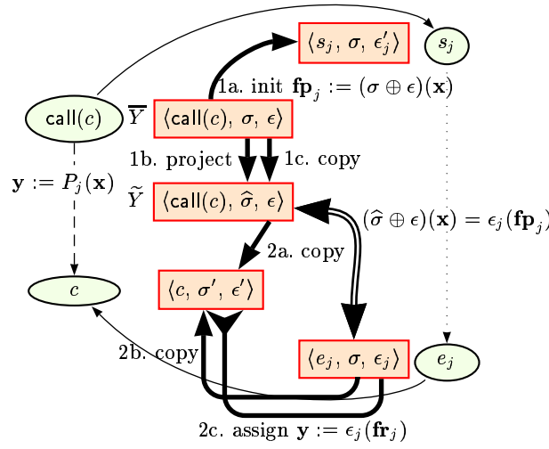
Figure 10: Abstract Postcondition for Procedure Call (1) and Return (2)
