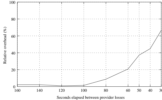
Figure 4: Relative overhead due to the volatility of providers for a sequence lock-put-unlock , with respect to a stable system.
