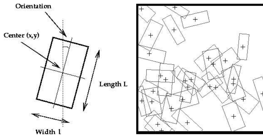
Figure 5: Parameterization of a rectangle and realization of a uniform Poisson point process of rectangles with mean 20.
