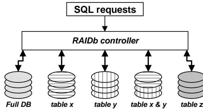
Figure 4. RAIDb-2 overview
