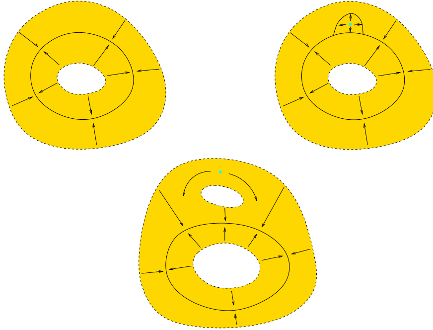
Figure 2: The gold region on the upper left corner deformation retracts on the bold curve. This is not true for the two other cases, since the gold region has to be torn to be collapsed on the bold curve (light blue points).
