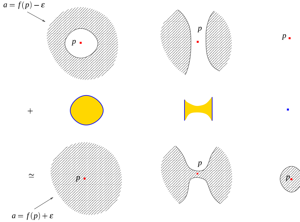
Figure 1: Smooth Morse theory in 2D.
