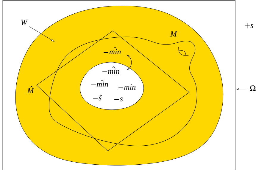
Figure 6: Condition 2'. and 4. are needed.
