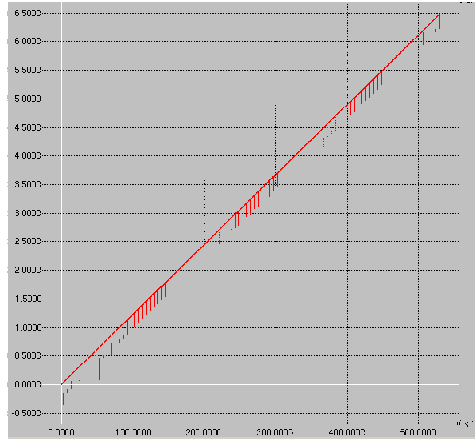
Figure 5: A clock drift (y-axis: difference of the local times) during 14h30 (x-axis: packet number)
