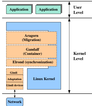
Figure 1: Kerrighed architecture
