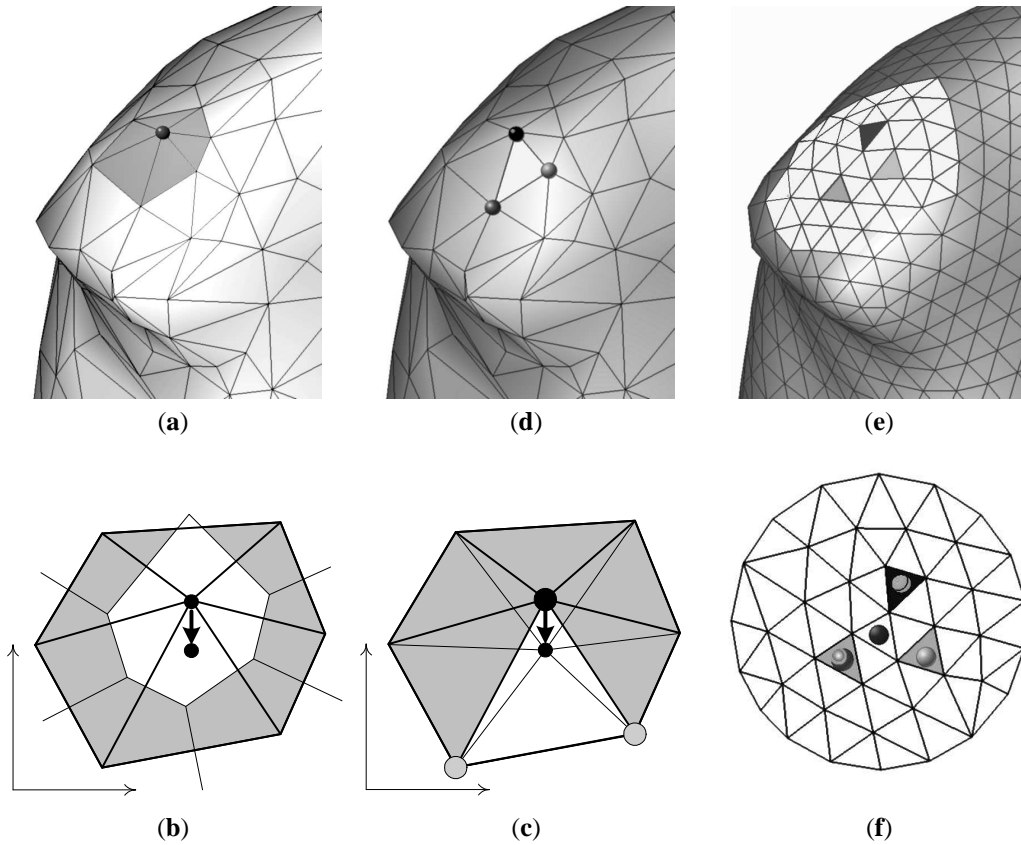
Figure 2: Vertex relocation. (a) A vertex v of the mesh to be relocated. The faces of the sub-mesh \mathcal{S}(v) are dark-grey. (b) \mathcal{S}(v) is mapped onto the plane and the Voronoi cell of v is constructed. The new vertex location is a weighted centroid of the cell. (c) The triangle containing the new location. (d) The corresponding triangle in the mesh \mathcal{M} . (e) The highlighted vertices in (d) correspond to three faces of the original mesh \mathcal{M}_O . (f) A patch containing all these faces of \mathcal{M}_O is constructed and then parameterized. The new location of v in the patch is computed using the corresponding barycentric coordinates of the 2D mapping (c).
