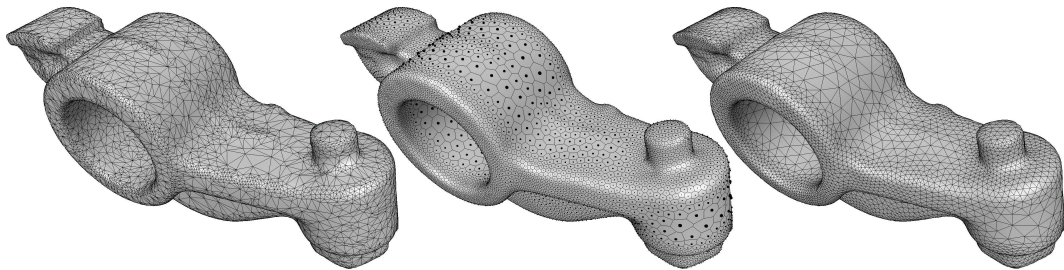
Figure 4: Left: original. Middle: centroidal tessellation. Right: curvature-adapted remeshing.
