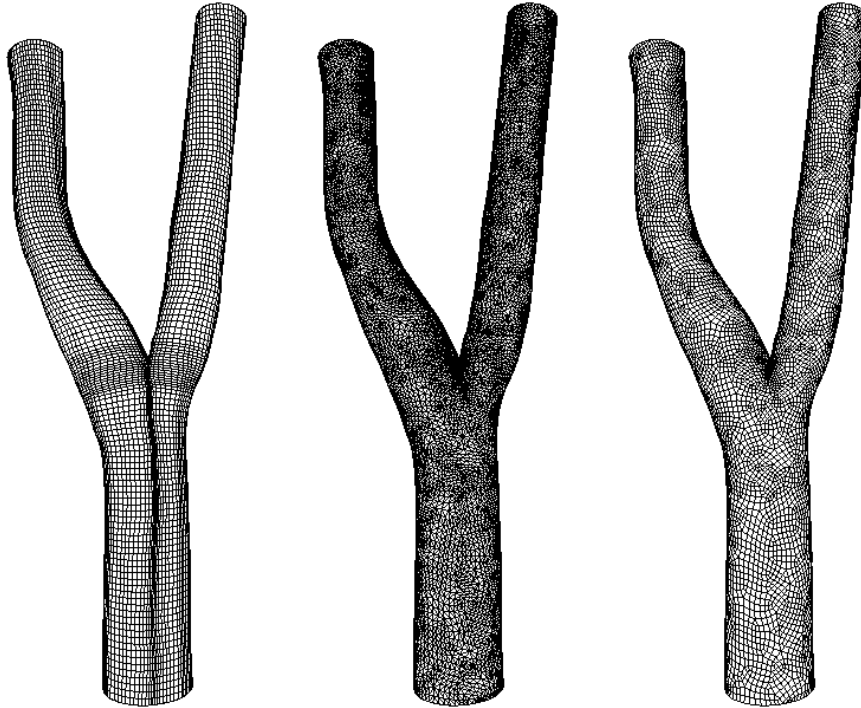
Figure 1: Left: hexahedral mesh (by courtesy of K. Perktold and D. Liesch), center: tetrahedral mesh, right: quadrilateral mesh.
