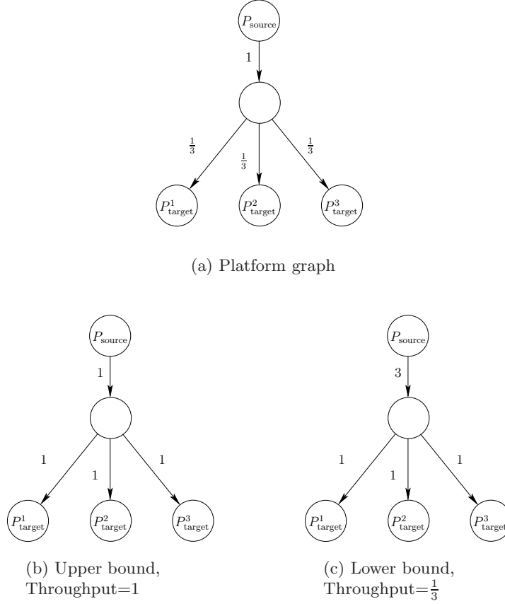
Figure 5: The distance between the lower and the upper bound may be |\mathcal{P}_{\text{target}}|
