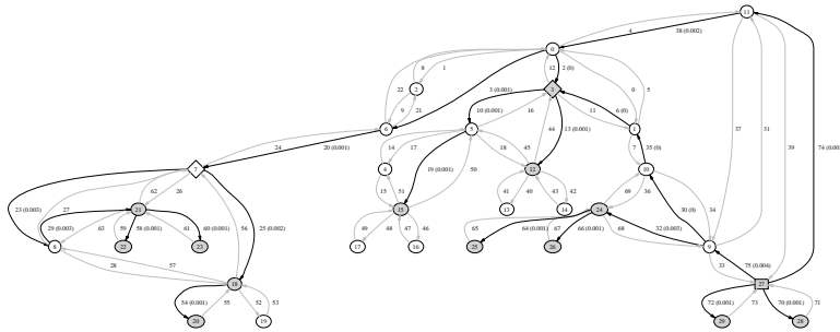
(c) Transfers involved in the Multisource MC solution. Edges are labeled with the quantity of messages transferred within one time-unit. Secondary sources (nodes 7 and 3) have a diamond shape.
