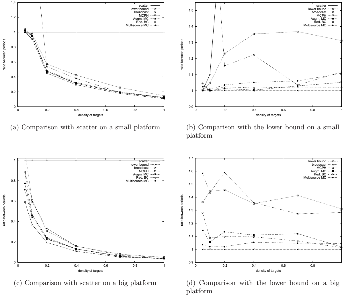
Figure 11: Comparison on the heuristics on two type of platforms
