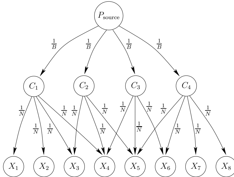
Figure 2: Instance \mathcal{I}_2 of COMPACT-MULTICAST obtained from the reduction of the following instance \mathcal{I}_2 of MINIMUM-SET-COVER: X = \{X_1, \dots, X_8\} , C = \{\{X_1, X_2, X_3, X_4\}, \{X_3, X_4, X_5\}, \{X_4, X_5, X_6\}, \{X_5, X_6, X_7, X_8\}\} .
