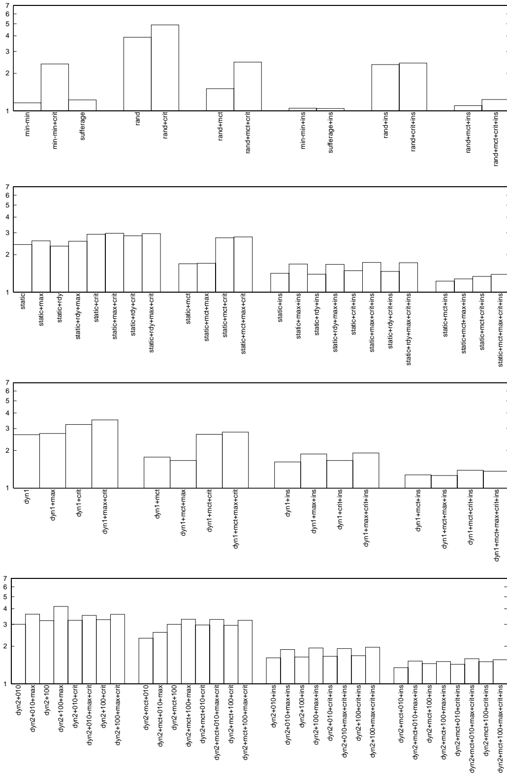
Figure 11: Relative performances of the schedules produced by the different heuristics for task graphs of type Partitioned . Average on three communication to computation ratios, and three types of platform graphs.
