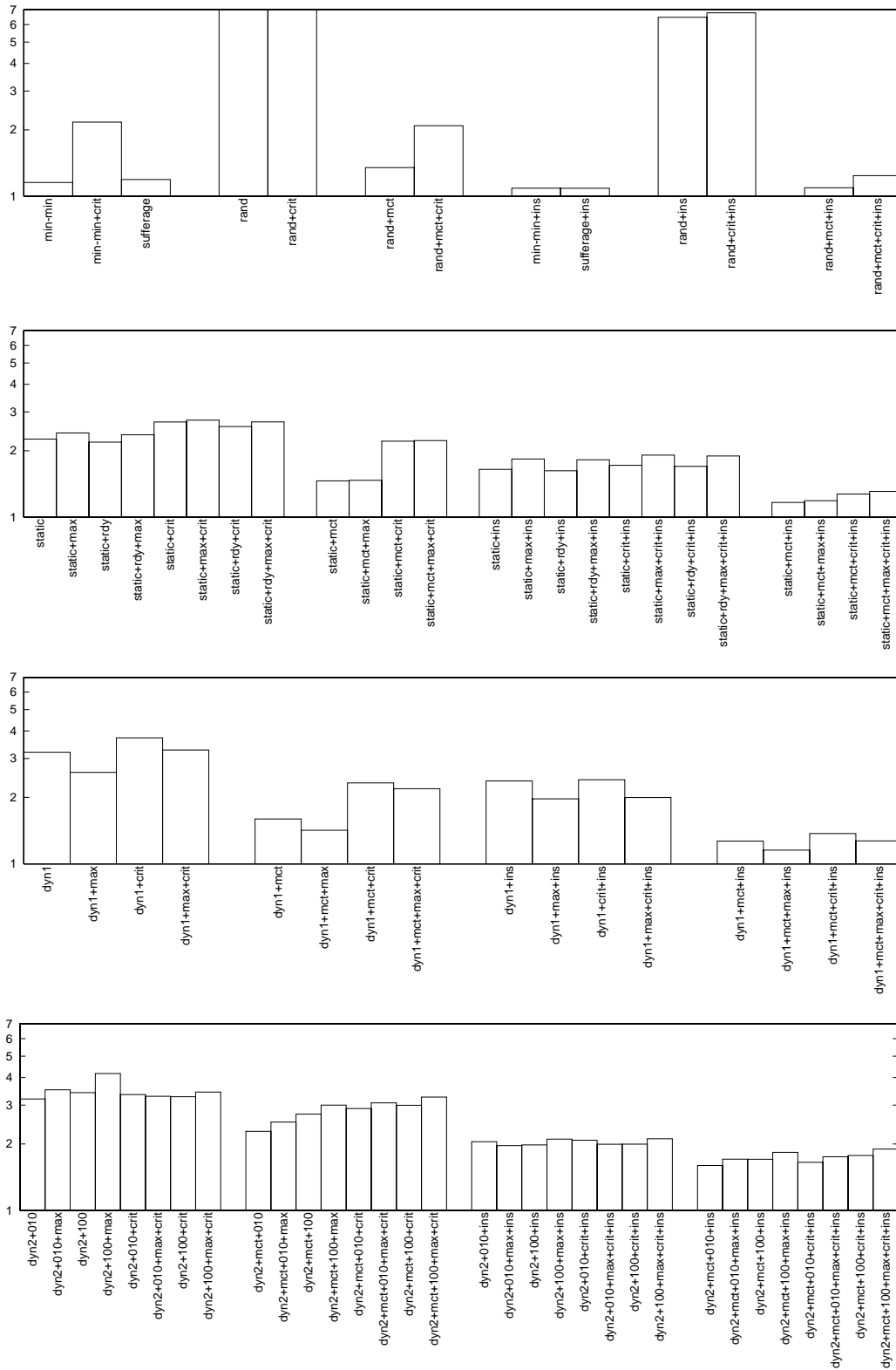
Figure 13: Relative performances of the schedules produced by the different heuristics for communication to computation ratio of 0.1. Average on four types of task graphs, and three types of platform graphs.
