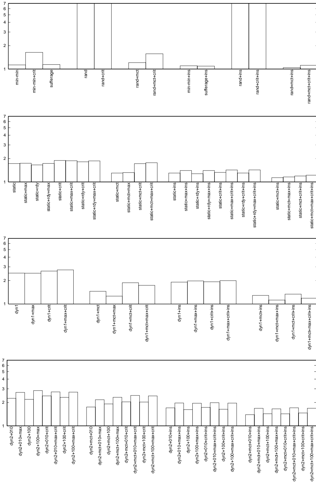
Figure 17: Relative performances of the schedules produced by the different heuristics for platform graphs of type Random Tree . Average on four types of task graphs, and three communication to computation ratios.
