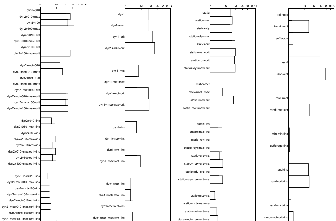
Figure 11: Relative performances of the schedules produced by the different heuristics for task graphs of type Partitioned . Average on three communication to computation ratios, and three types of platform graphs.
