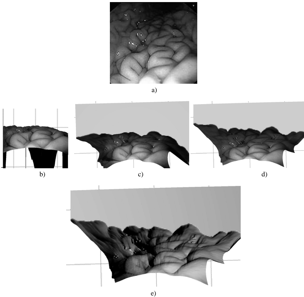
Figure 7: Reconstruction of a normal stomach: a) Original image of a normal stomach [size \simeq 200 \times 200 ]; b) surface recovered from a) by our generic algorithm with the orthographic model ( \mathbf{L} = (0, 0, 1) ); c) surface recovered from a) by our generic algorithm with the perspective model with the light source at infinity ( \mathbf{L} = (0, 0, 1) ); d) surface recovered from a) by our generic algorithm with the perspective model and with the light source located at the optical center; e) surface d) visualized with a different illumination.
