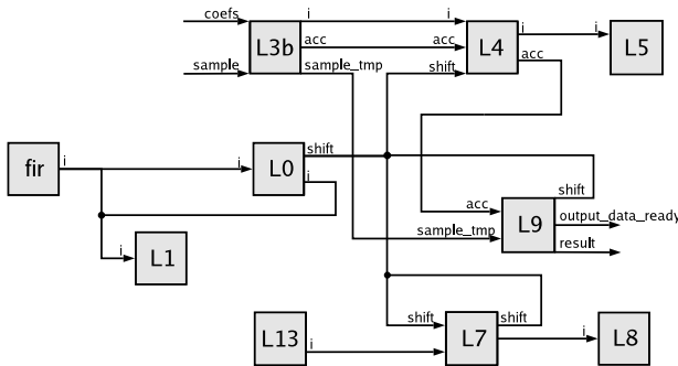
Figure 14: Data Flow of the FIR
