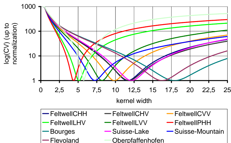
Figure 3.5: Logarithmic plot of the CV functional for all the considered 11 images (the 11 functionals have been rescaled in the range [1, 1000] only for visualization purposes).
