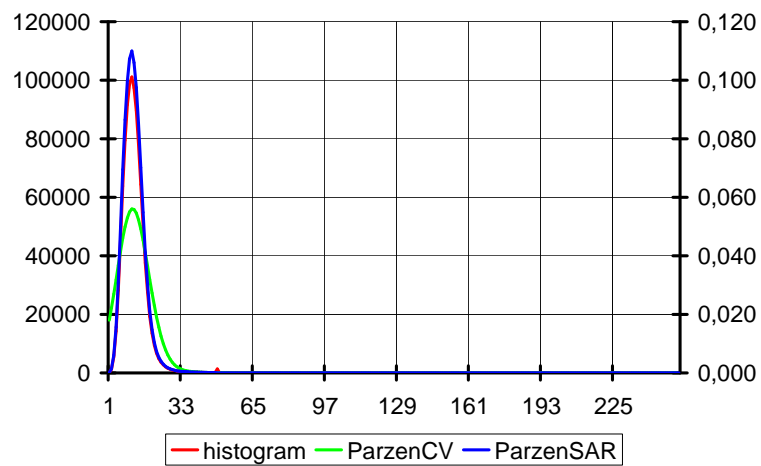
Figure C.11: Plot of the image histogram and of the Parzen PDF estimates for the “Oberfaffenhofen” data set.
