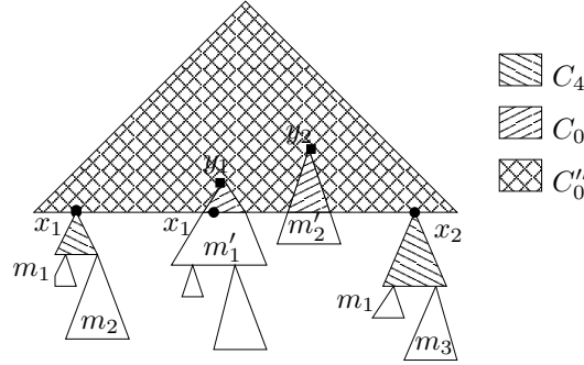
Fig. 2. Transforming C_0\theta into C_0''[C_1^0[M_1, \dots, M_k], \dots, C_r^0[M_1, \dots, M_k], M_{r+1}'', \dots, M_n'', M_1, \dots, M_k] .
