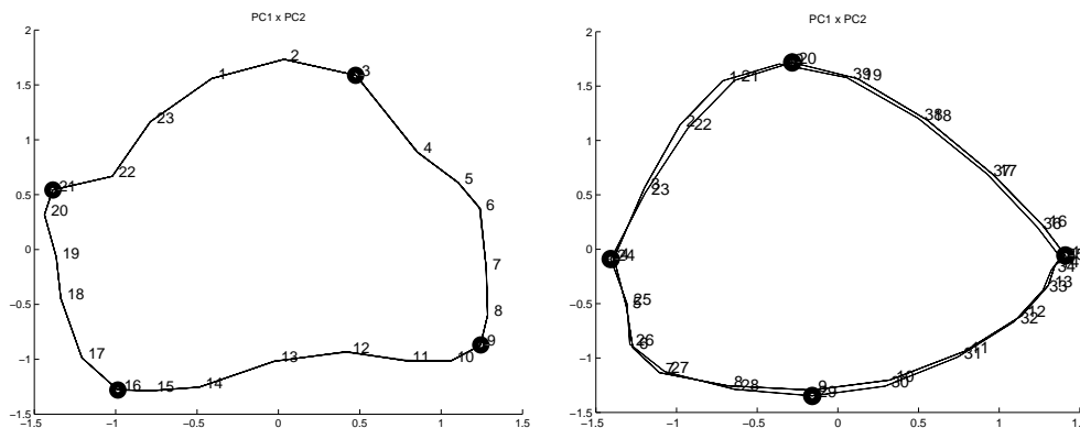
Figure 3: PC1(t) \times PC2(t) : PC projections across time for two synthetic sequences of horse: canter and walk. Frames are numbered for one cycle. Circles are selected examples by the condition number criterion.
