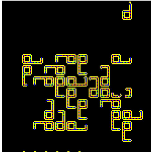
Figure 4: Sayama's SDSR-Loop
