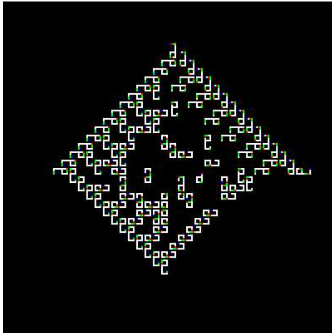
Figure 7: PSDSR-Loop
