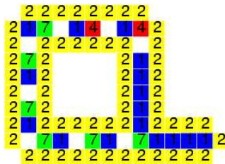
Figure 3: SR-loop
