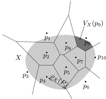
Figure 2: Voronoi tessellation
