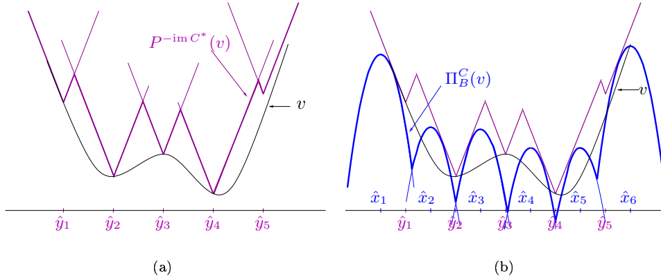
Figure 1: Example illustrating max-plus and min-plus projectors
