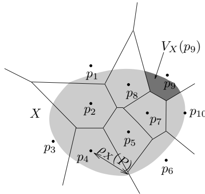
Figure 2: Voronoi tessellation
