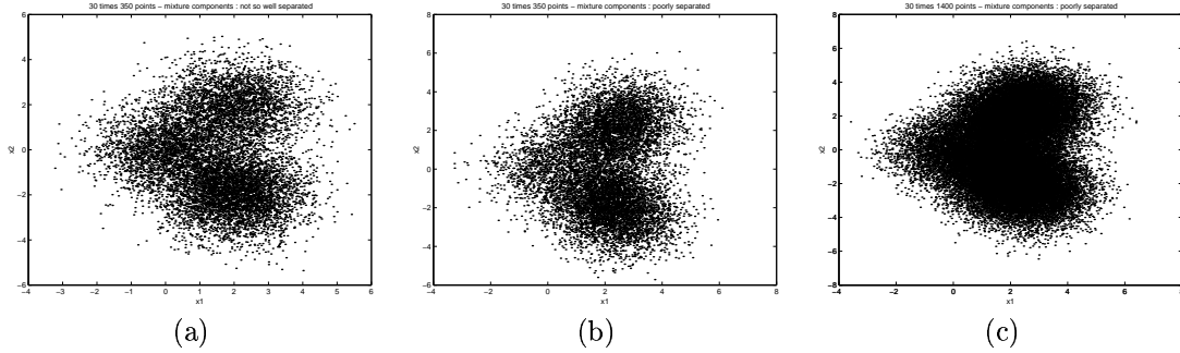
Figure 2: (a) Simulated data from 30 HMCs of length 350 with K = 3 hidden states; (b) Simulated data from 30 HMCs of length 350 with K = 5 hidden states; (c) Simulated data from 30 HMCs of length 1,400 with K = 5 hidden states.
