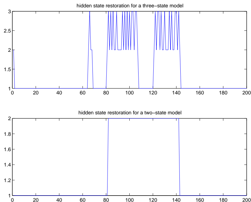
Figure 5: Hidden state restoration for the heart rate variability dataset with the Viterbi algorithm (applied to the first 200 points). Top: three-state HMC model. Bottom: two-state HMC model.
