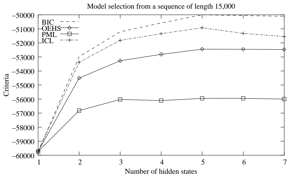
Figure 3: The behaviour of criteria OEHS, BIC, ICL and PML for a sequence of length 15,000 simulated using a five-state HMC
