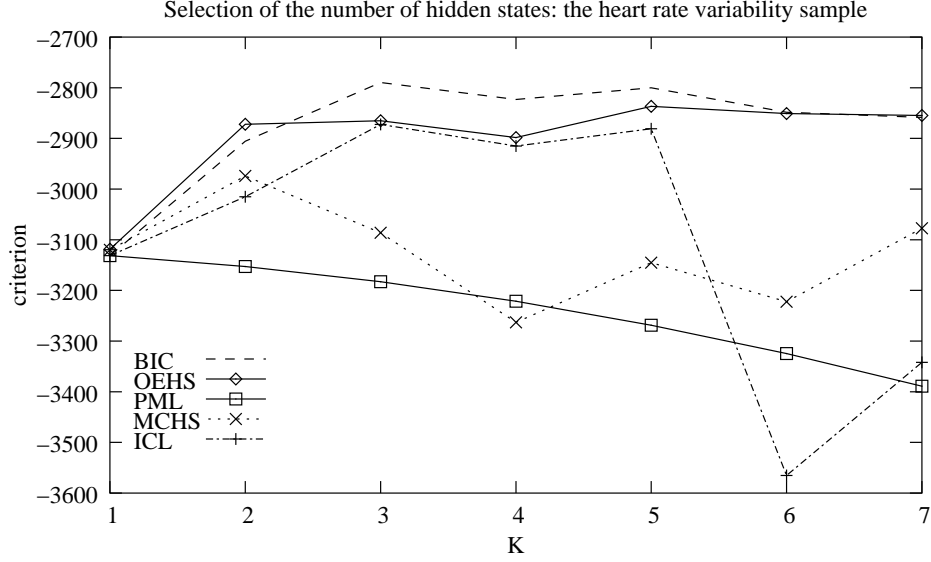
Figure 4: Model selection for the heart rate variability sample. The values of the criteria OEHS, MCHS, BIC, PML and ICL are represented as a function of the number of hidden states K .
