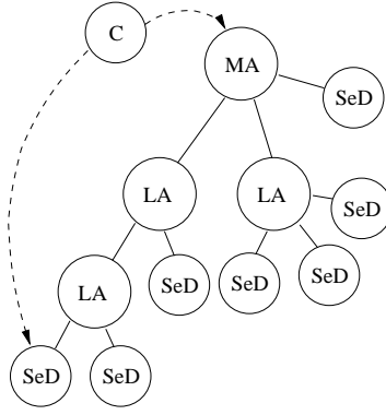
Figure 2: DIET hierarchical organization.
