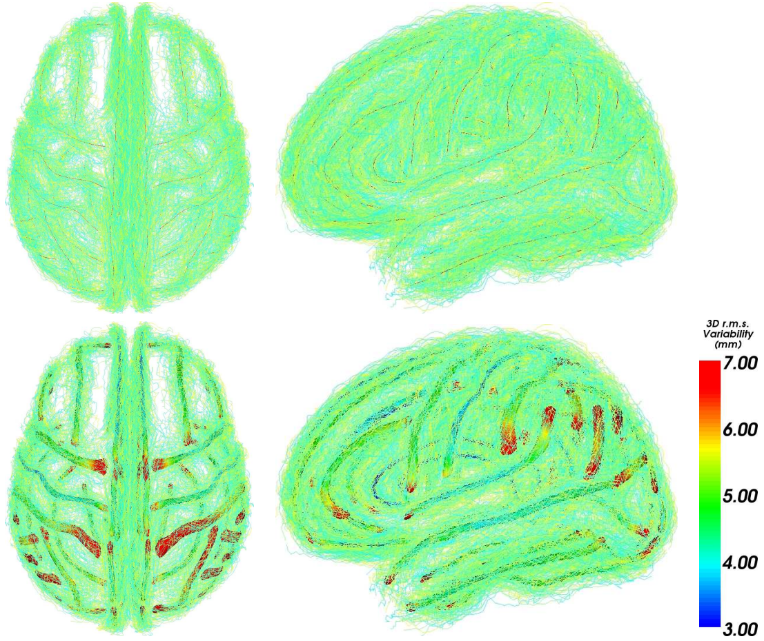
Figure 2: Sulcal variability. Top: The sulcal lines alone. Mean curves are shown in red, and traces from 98 healthy normal individuals are displayed in green and yellow. Bottom: Covariance matrices (ellipsoids at one \sigma ) are overlapped at regularly sampled spatial positions along the mean sulci. The color codes for the trace: Note that tensors close to the sulci extremities are larger.
