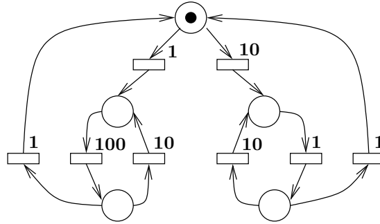
Figure 5: Example of a Petri net where the maximum throughput with Bernoulli routing can be higher than with the race policy.
