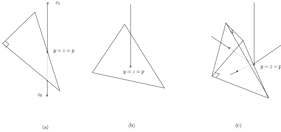
Figure 2: Points p which are topologically regular although \nabla d_K(p) = 0 (a) \partial O^* \cap \text{RelInt}(O) \neq \emptyset (b) \text{RelInt}(O^*) \cap \partial O \neq \emptyset (c) Voronoi vertex on an edge. Signature of tetra is (4, 5, 2, 0)
