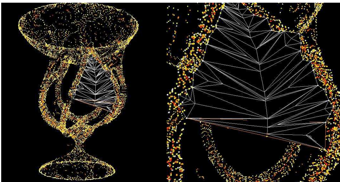
Figure 12: Left: far view of the critical points and of the stable manifold with 264 triangles. Right: closeup.
