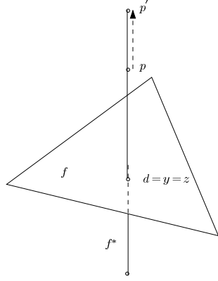
Figure 3: Flow segments E-E-\{V, \infty\} : from a Voronoi edge f^* dual of a critical Delaunay triangle f .
