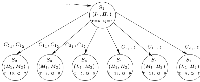
Figure 14: Configurations reachable in one step from S_1 , upon reception of (Req_1 and Go_1) and in the absence of Stop_2 , according to controllables C_{k_1}, C_{k'_2} , with weights of cost and quality.
