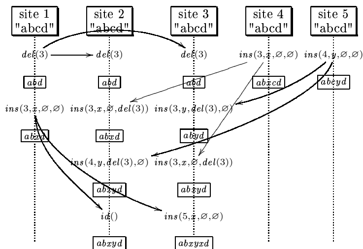
Figure 6: Suleiman counter example
