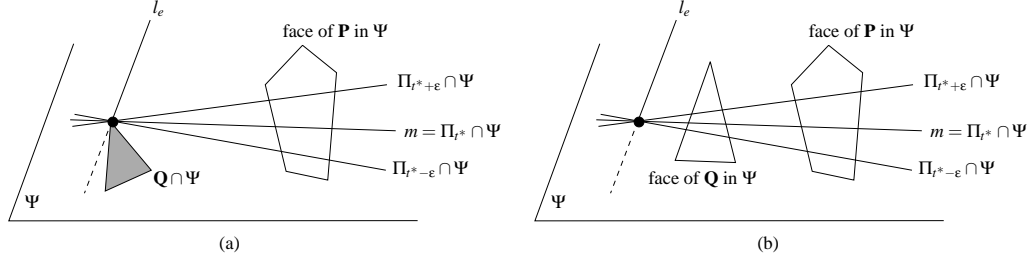
Figure 9: m is tangent to \mathbf{P} along a face in \Psi and (a) to \mathbf{Q} \cap \Psi only on l_e or (b) to \mathbf{Q} along a face in \Psi .
