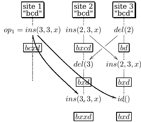
Figure 13: IMOR counter example (3 sites)
