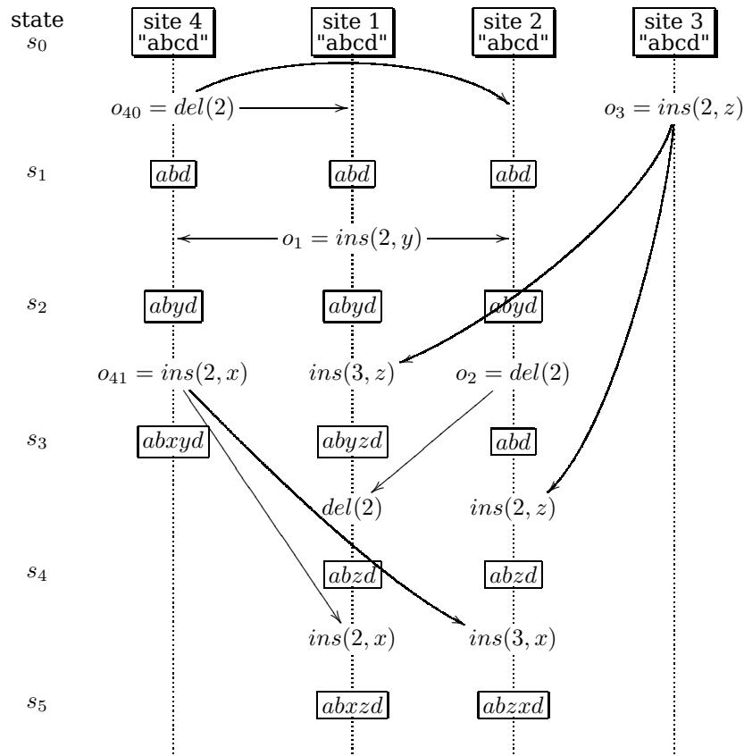
Figure 20: SDT counter-example
