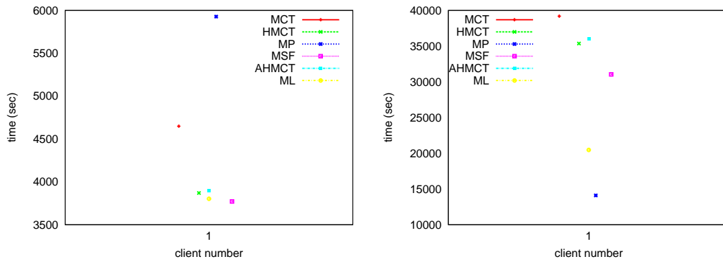
Figure 19. Scenario (e'): makespan and sumflow results
