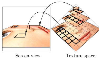
Figure 2: The pyramidal structure of texture space.
