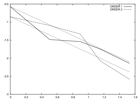
(f) Transcritical flow with shock - Convergence rate
