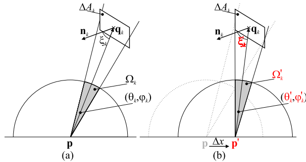
Figure 3: Gradient computation by displacing the hemisphere center from \mathbf{p} to \mathbf{p}' ((a) before and (b) after the displacement). The quantities changing with the displacement are (shown in red): sample ray direction (\theta_k, \phi_k) ; the solid angle \Omega_k associated with this sample; the angle \xi_k between the sample direction and the surface normal at the hit point \mathbf{q}_k . Neither the hit point \mathbf{q}_k nor the area \Delta A_k visible through \Omega_k change with the displacement.
