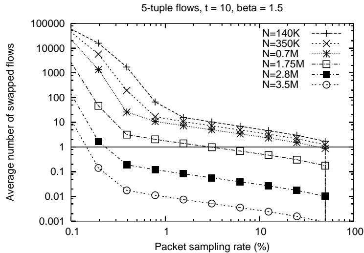
Figure 8: Performance of sampling with 5-tuple flows varying the total number of flows
