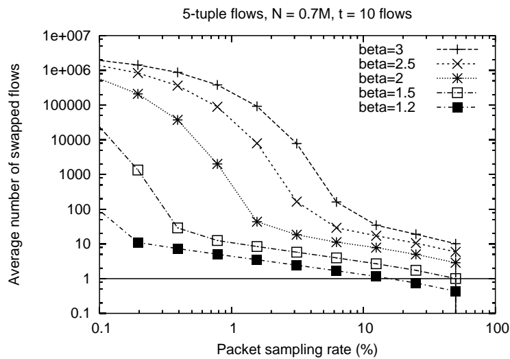
Figure 6: Performance of sampling with 5-tuple flows varying the flow size distribution
