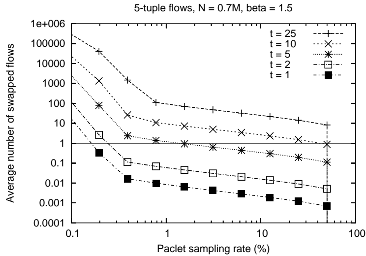
Figure 4: Performance of sampling with 5-tuple flows varying the number t of top flows of interest
