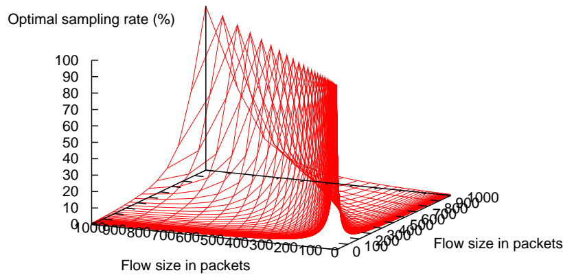
Figure 2: Optimal sampling rate (normal scale)
