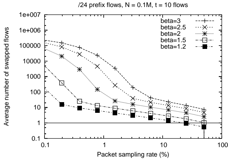
Figure 7: Performance of sampling with /24 prefix flows varying the flow size distribution
