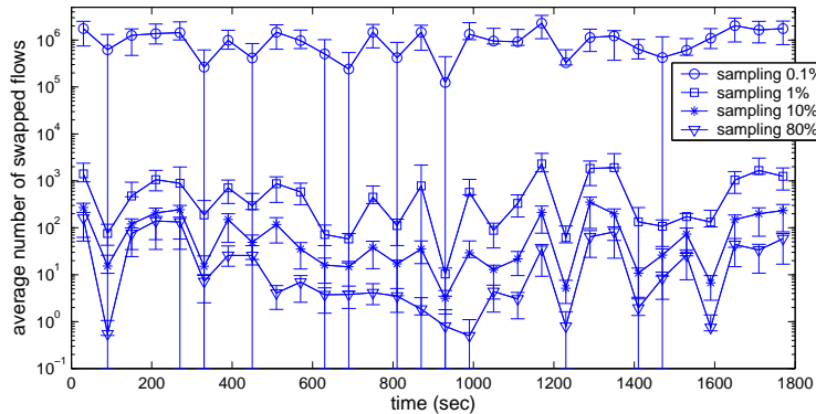
Figure 16: Performance of ranking vs. time, 5 tuple, top 10 flows, Abilene network
