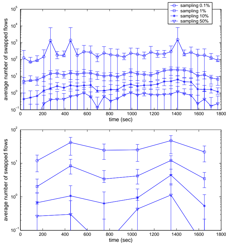
Figure 13: Performance of ranking vs. time, /24 prefix, top 10 flows
