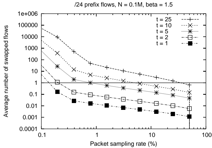
Figure 11: Detection of the largest flows (/24 prefix)
