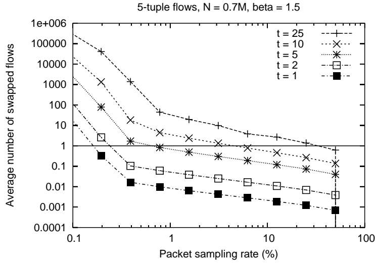
Figure 10: Detection of the largest flows (5-tuple)
