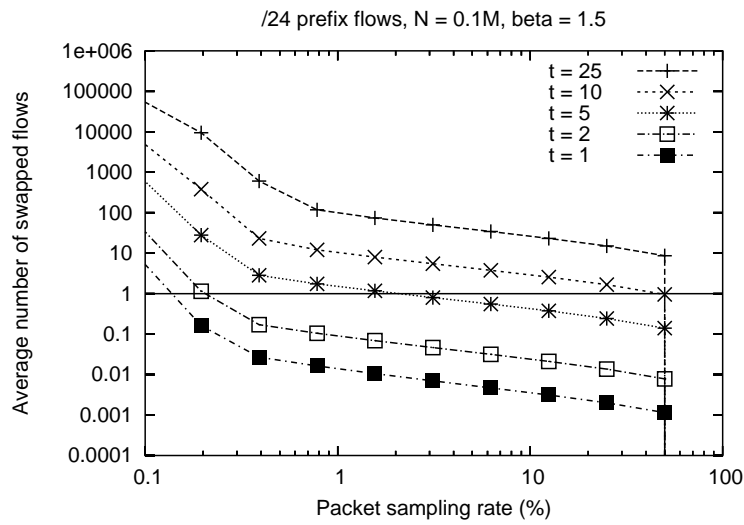
Figure 5: Performance of sampling with /24 prefix flows varying the number t of top flows of interest
