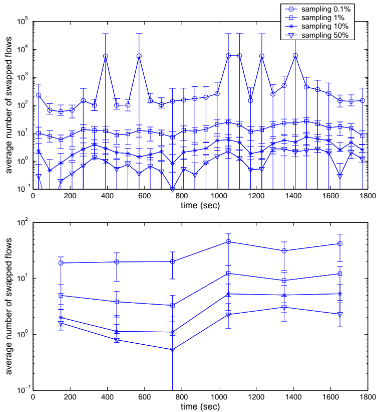
Figure 12: Performance of ranking vs. time, 5-tuple, top 10 flows
