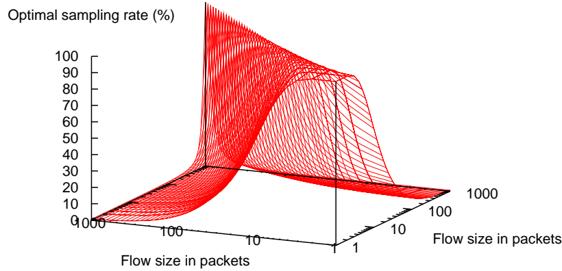
Figure 1: Optimal sampling rate (log scale)
