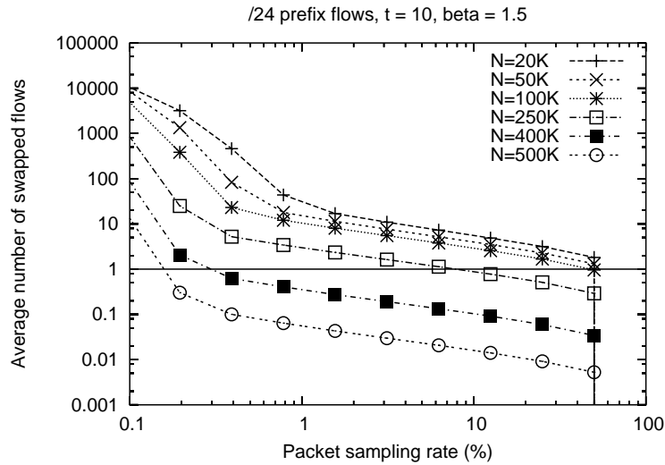
Figure 9: Performance of sampling with /24 prefix flows varying the total number of flows
