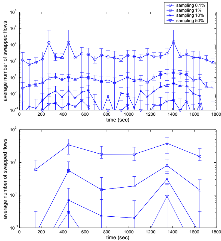
Figure 15: Performance of detection vs. time, /24 prefix, top 10 flows
