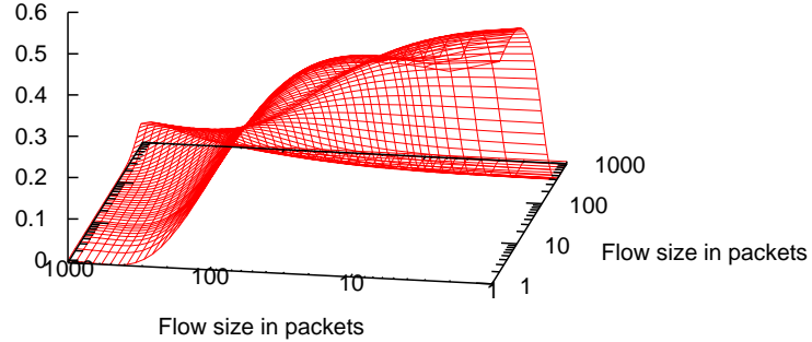
Figure 3: Gaussian approximation - absolute error, sampling rate 1%
