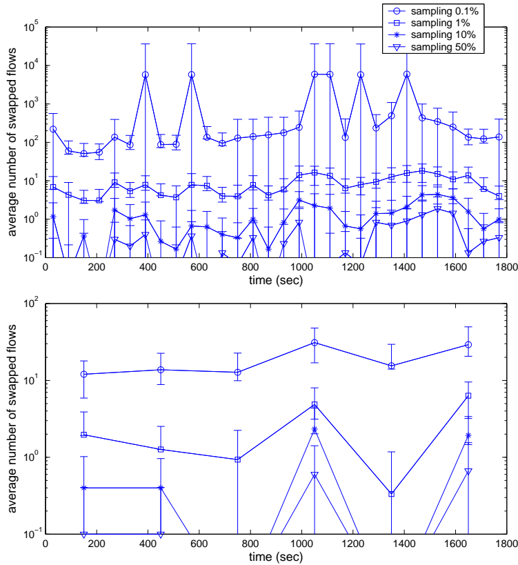
Figure 14: Performance of detection vs. time, 5-tuple, top 10 flows
