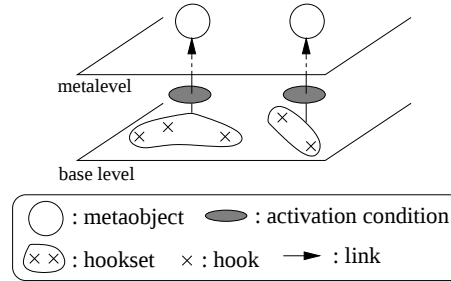
Figure 5: The hookset model for partial behavioral reflection.
