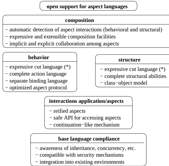
Figure 3: Summary of identified requirements for a versatile AOP kernel.
