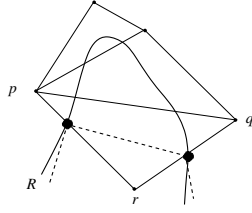
Figure 22: Double crossing with an edge correctly processed: the ridge (solid curve) is shortened (dashed polyline)
