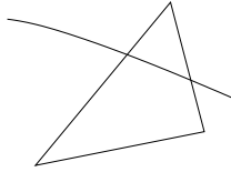
Figure 17: Two ridge crossings
