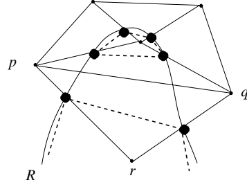
Figure 23: Double crossing with an edge leading to an erroneous topology: the ridge (solid curve) is split (dashed polyline)
