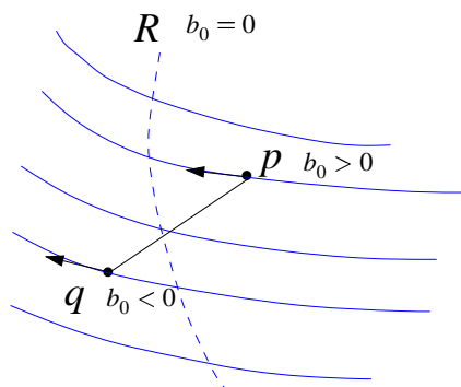
Figure 7: The image of an edge, a blue ridge and the blue principal foliation
