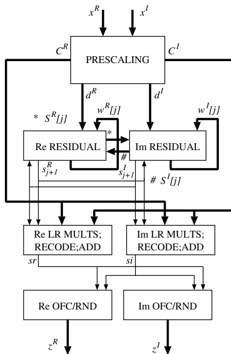
Figure 2: Overall scheme for computing complex square root.
