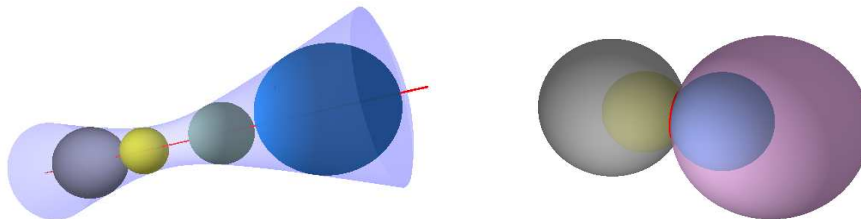
Figure 1: Two examples of quadruples of spheres with infinitely many common tangents.
