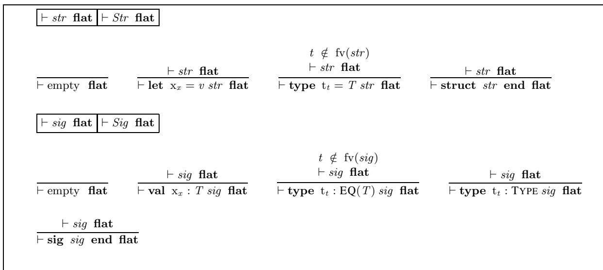
Figure 8: Typing Rules – flat predicates
