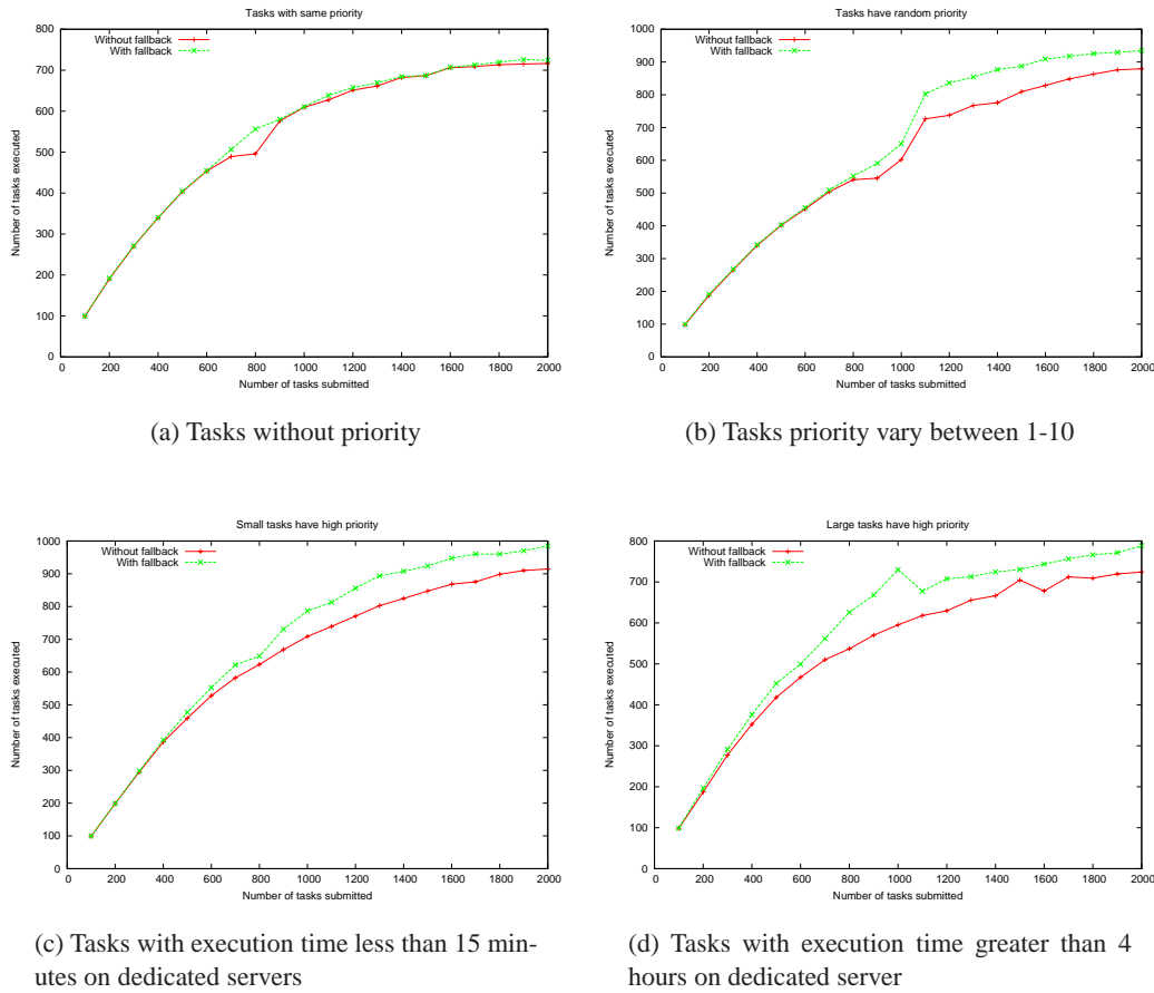
Figure 4: Comparison of tasks executed with and without fallback.
