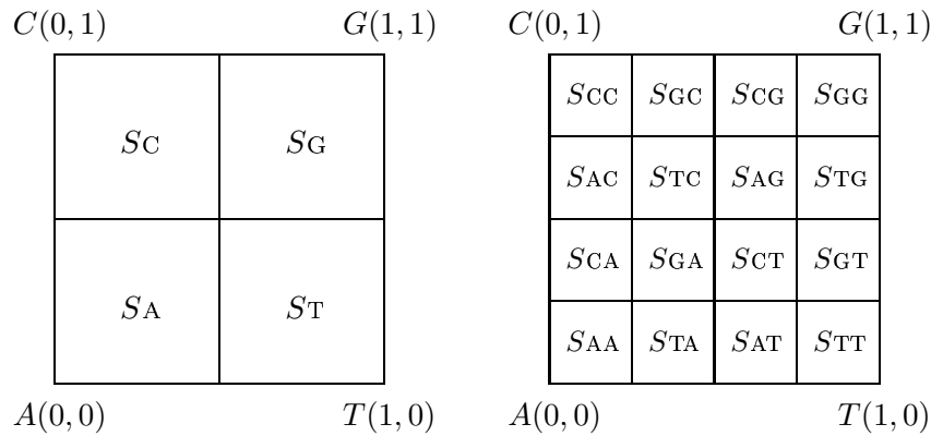
Figure 1.1: Definitions of the squares corresponding to nucleotides (left) and dinucleotides (right) for the CGR on [0, 1]^2 .
