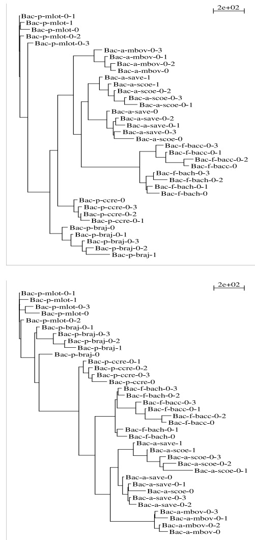
Figure 4.4: Unrooted lineage trees built using the NJPLOT method from the dinucleotide relative abundance differences (top) and the CGR-based relative abundance differences of (bottom) for all the sequences of Bacteria. With the CGR, the 3 groups Firmicutes , Pro bacteria and Actinobacteria are demarcated, whereas Firmicutes appears as a family of Actinobacteria in the top tree.
