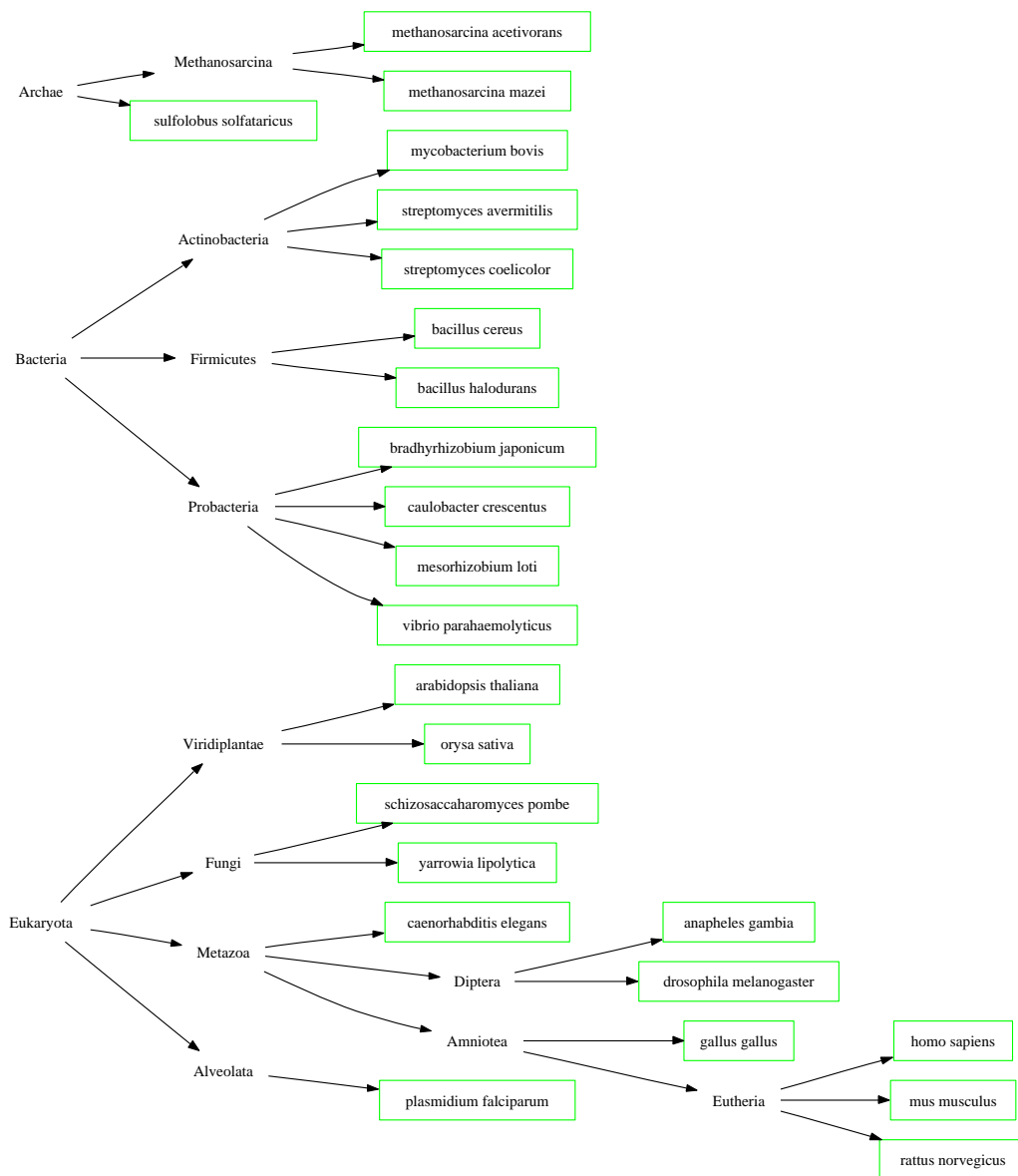
Figure 4.1: Lineage tree of the species used in the experiments.
