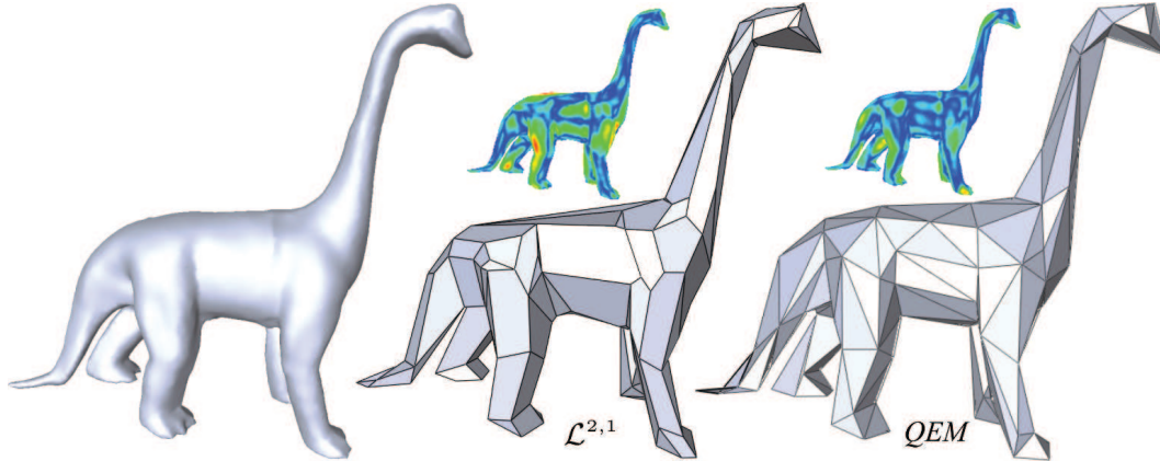
Figure 14: (Left) Dinosaur model; (Center) \mathcal{L}^{2,1} -approximation; (Right) Results for QEM [GH98] with same number of edges. Note that our approach reproduces the “highlights” (see neck), with a symmetric Hausdorff error 18% better (as measured by [ASCE02]).
