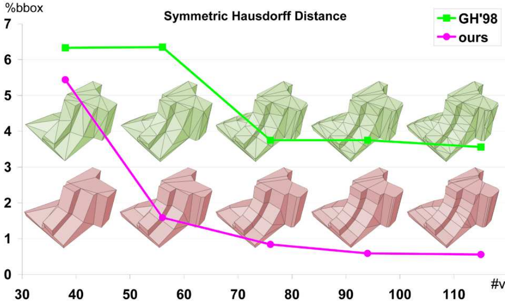
Figure 15: Comparison of the Hausdorff error for QEM [GH98] and for our \mathcal{L}^{2,1} technique, for equal number of vertices (a comparison using equal number of edges leads to an extremely similar curve).
