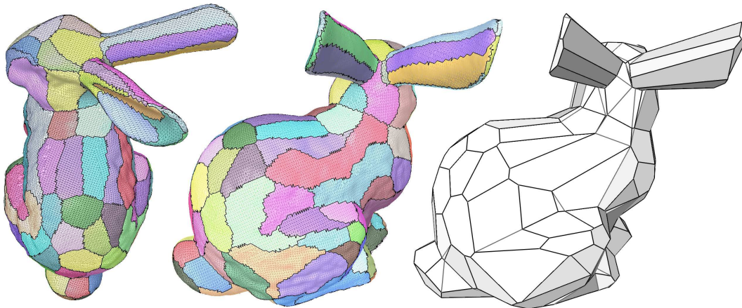
Figure 3: Bunny: (left and center) \mathcal{L}^{2,1} -optimized geometric partitioning; (right) Anisotropic polygonal mesh deduced from the partition. Notice the stretching of the elements on the ears.
