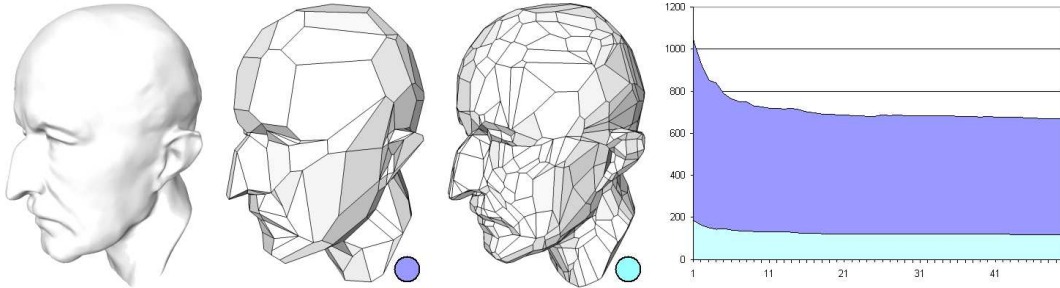
Figure 10: Max Planck: For the two optimized approximations (130 and 300 proxies resp.), we show the associated curves of the \mathcal{L}^{2,1} -distortion error as a function of the number of Lloyd's iterations; as expected, a few iterations suffice to reach a much reduced distortion error.
