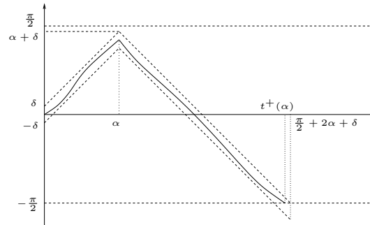
Figure 3: The graph of \theta^+(\cdot, \alpha) .
