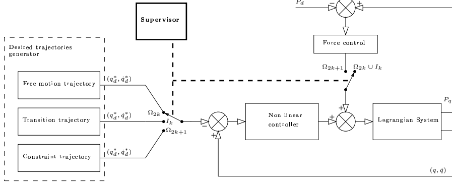
Figure 5: Structure of the controller
