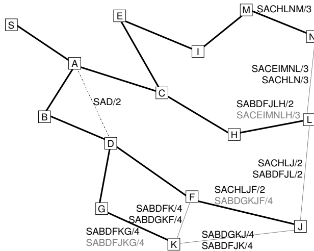
Figure 3: Result of First Round of Backup Multicast Tree Construction
