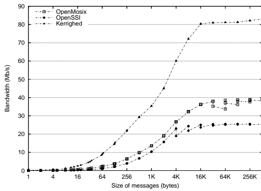
Figure 14: Pipe Bandwidth after both ends migrated on different nodes
