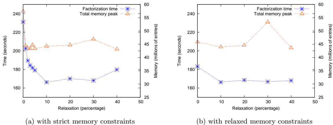
Figure 6: Influence of the memory relaxation on the factorization time and on the memory effectively used for matrix CONV3D64 on 128 processors.
