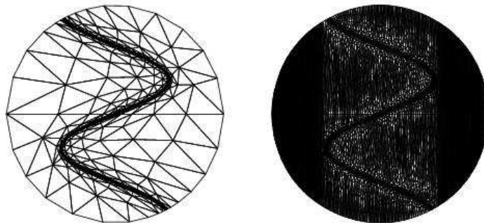
Figure 16: Representation of a function with the two options, L^\infty (left) and L^2 (right): corresponding meshes.
